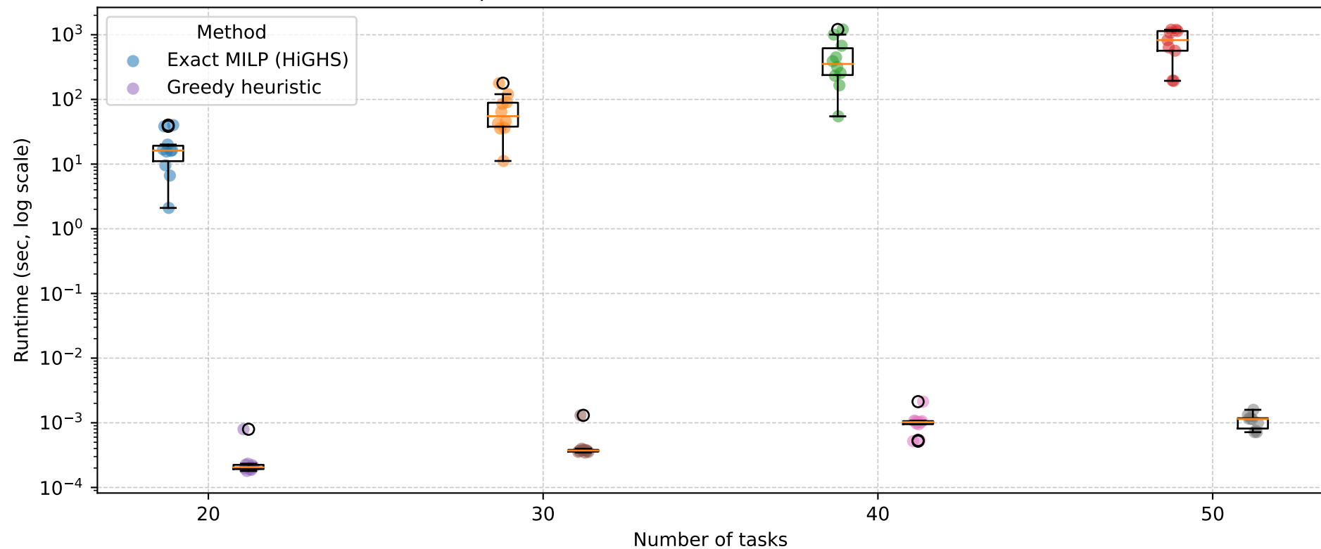
Distribution of computational runtime across TTAP instances - 6 Helos / 7 Areas
